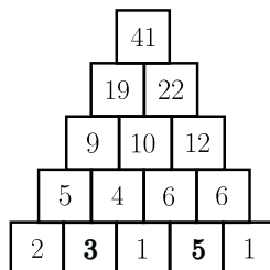
Obrázek 5: a = 2 a c = 1
