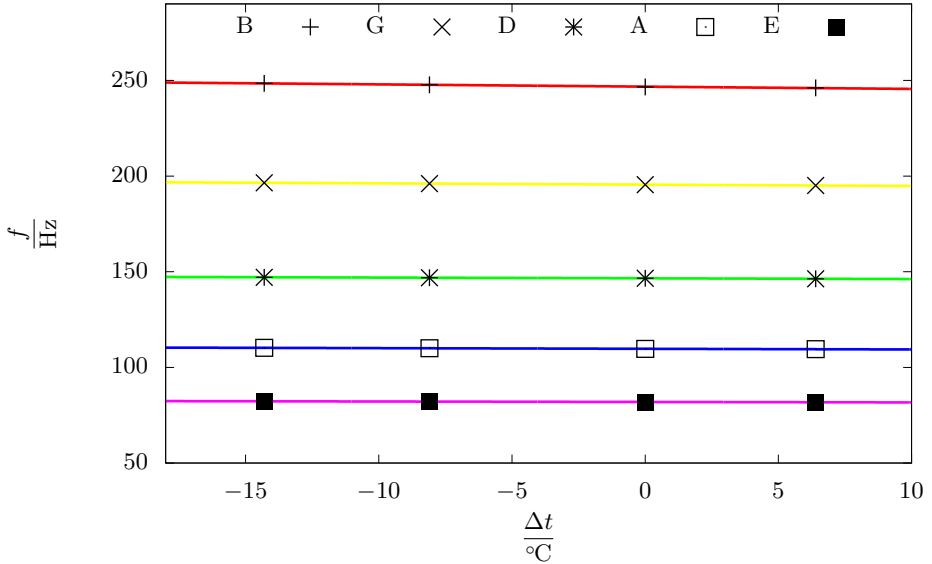
Figure 1: Dependence of the string frequencies on the temperature change. Due to the small changes in frequency, the dependencies look almost constant.
