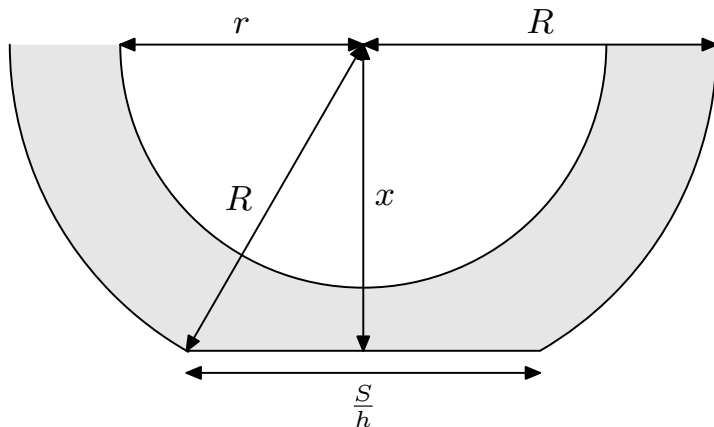
Figure 1: Sketch for the calculation of the distance x of the ground from the centre of the tire.
